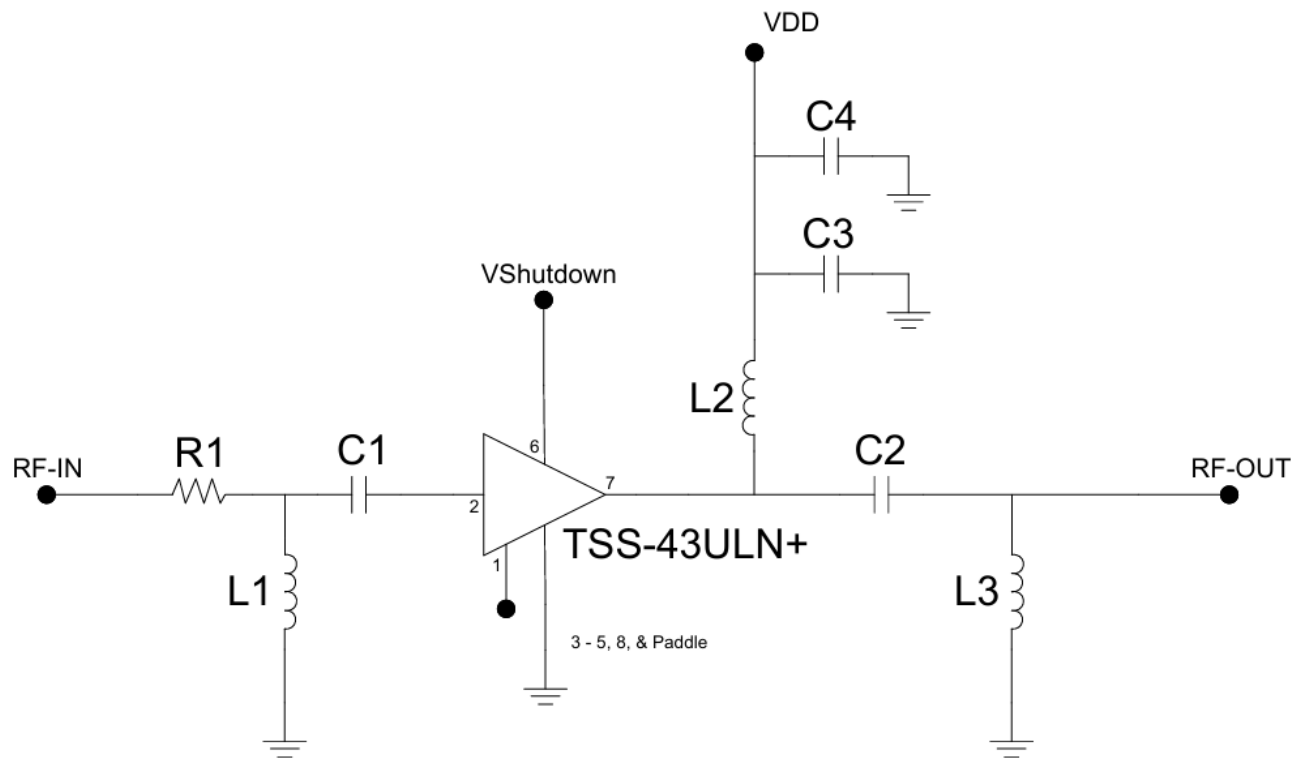
Figure 3. Schematic of the 1.5 – 1.6 GHz application circuit that includes the TSS-43ULN+ device.
