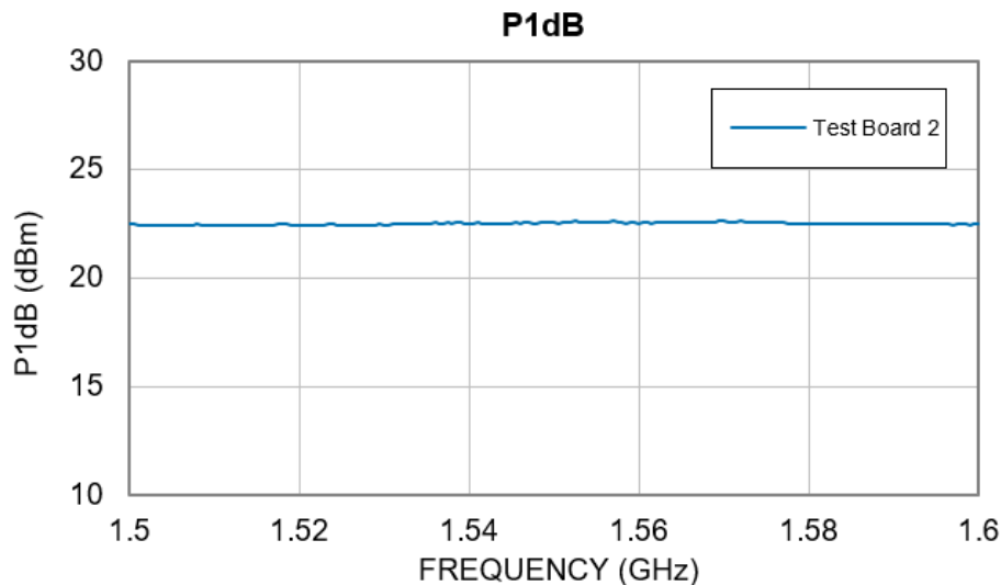
Figure 9. Measured P1dB.
