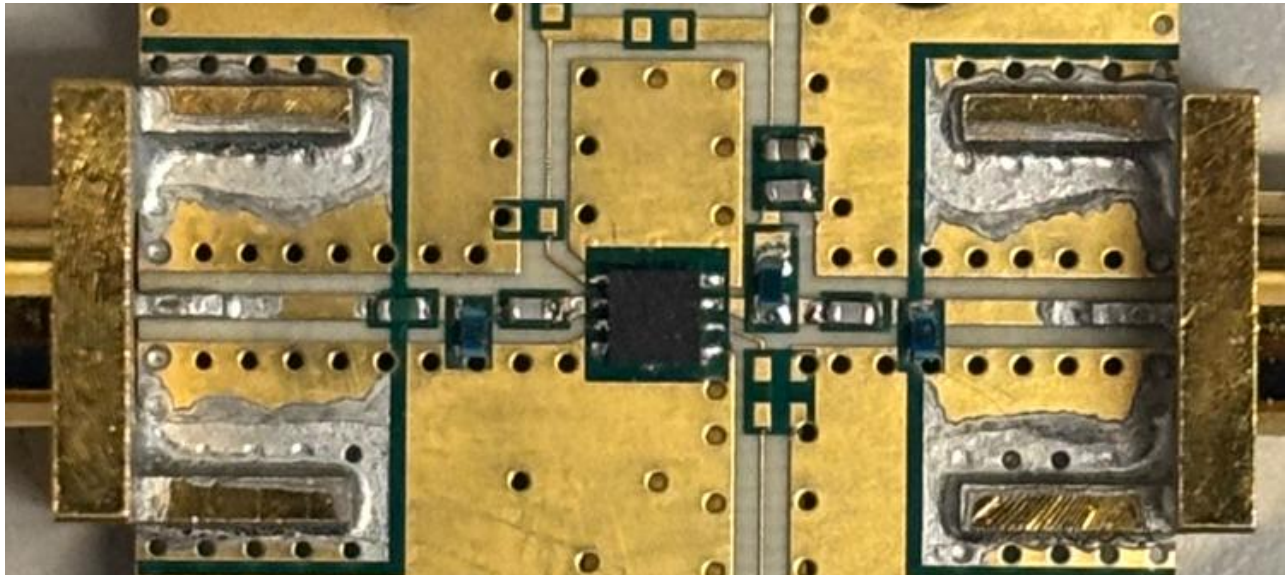
Figure 4. Fully assembled 1.5 – 1.6 GHz test board.
